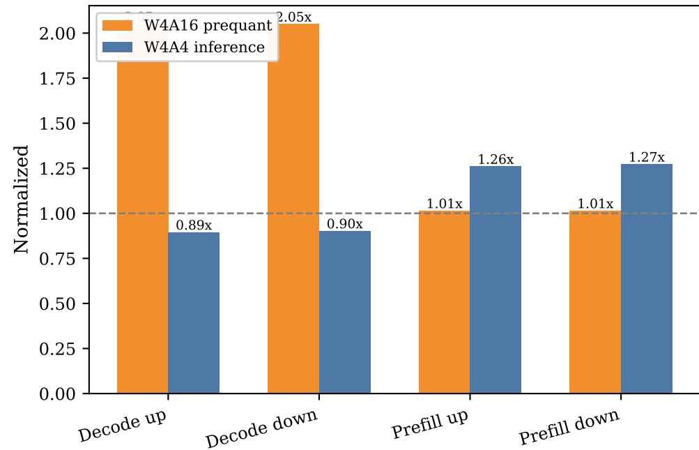
Energy vs FP16
